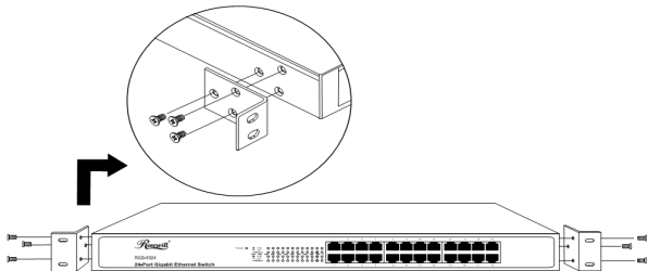
Figure 2-1 Rivet the "L" brackets onto the Switch
